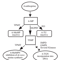
Figure 1. Metabolism pathway of azathioprine: competing pathways result in inactivation by TPMT or XO, or incorporation of cytotoxic nucleotides into DNA.
